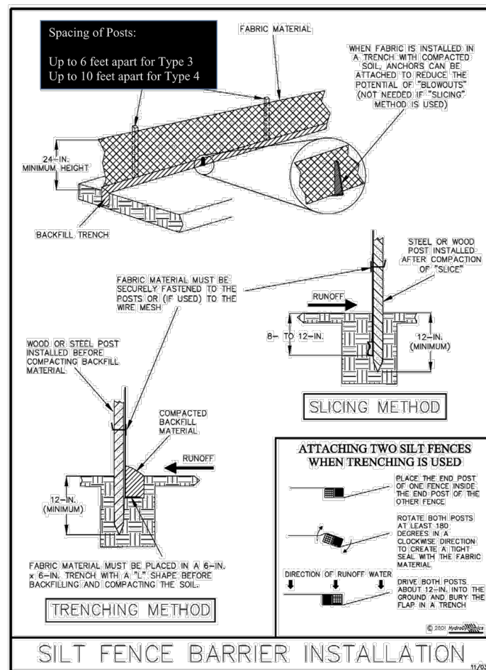
Figure V-2: Illustration of a Silt Fence Barrier Installation
