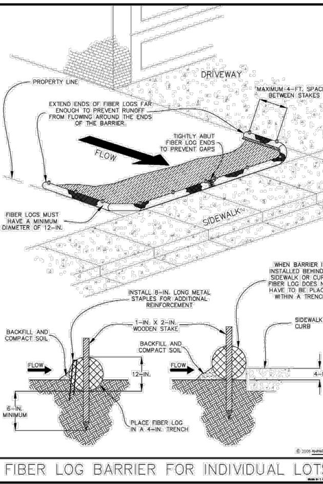
Figure V-5: Illustration of Fiber Log Barriers for Individual Lots
